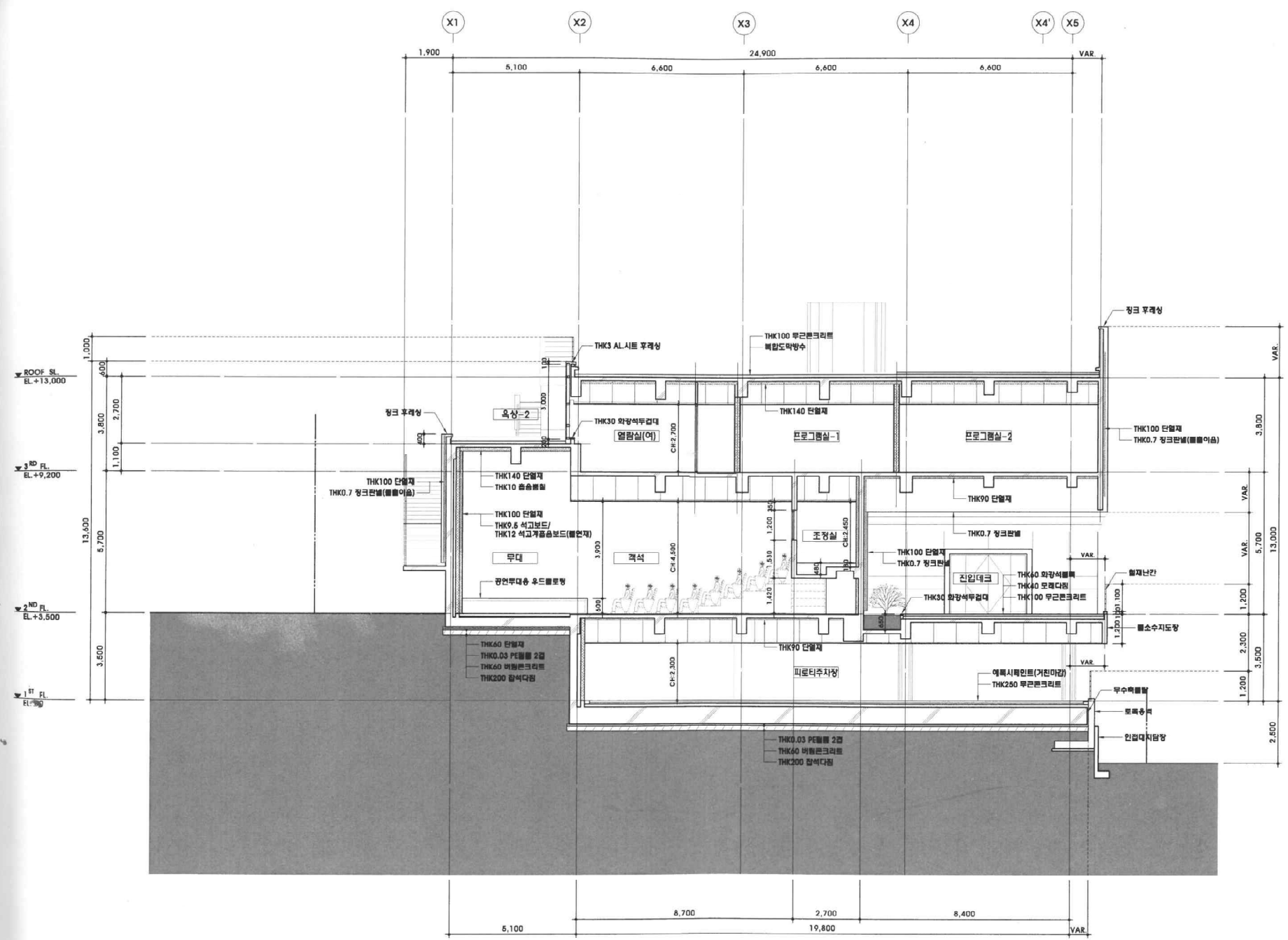
A 횡단면도-1 A3=1/150
